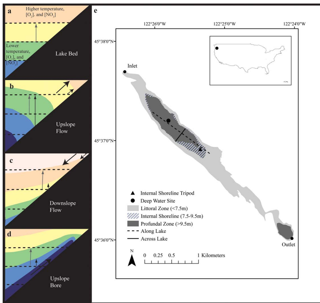
Fig. 1. (a–d) Cross-sections of the internal shoreline bottom boundary layer. Contour lines depict thermal stratification and associated chemical stratification during neutral flow (a), upslope flow (b), downslope flow (c), and in the presence of a thin internal bore (d). Near-bed stratification is reduced during upslope flow (b) and intensifies during downslope flow (c) relative to the stratification during neutral flow (a). Dotted lines and grey arrows in panels a–d indicate stratification contours during neutral flow; vertical black arrows in panels b–d show shear induced stratification contours; diagonal black arrows in panels b–d show direction of flow. Study site map (e) showing the locations of the internal shoreline tripod (▲) and deep-water (●) sampling station, as well as the profundal, littoral, and internal shoreline zones of Lacamas Lake. Black dot on insert map indicates the location of Lacamas Lake in Washington State.
