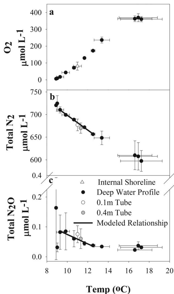
Fig. 7. Mean temperature plotted against mean O_2 (a), N_2 (b), and N_2O (c) at 11 depths from the deep water site on 8 June 2012 and 19 June 2012 (black circles), and from the 23-h sampling event (white and gray circles). Internal shoreline O_2 concentration measurements were made by an optical O_2 probe at z = 0.1 m (white circle in panel a). Internal shoreline N_2 and N_2O concentration measurements were made via tube sampling at 0.1 m (white circles in panels b and c) and 0.4 m (gray circles in panels b and c). Error bars represent 1 standard deviation from the mean.
