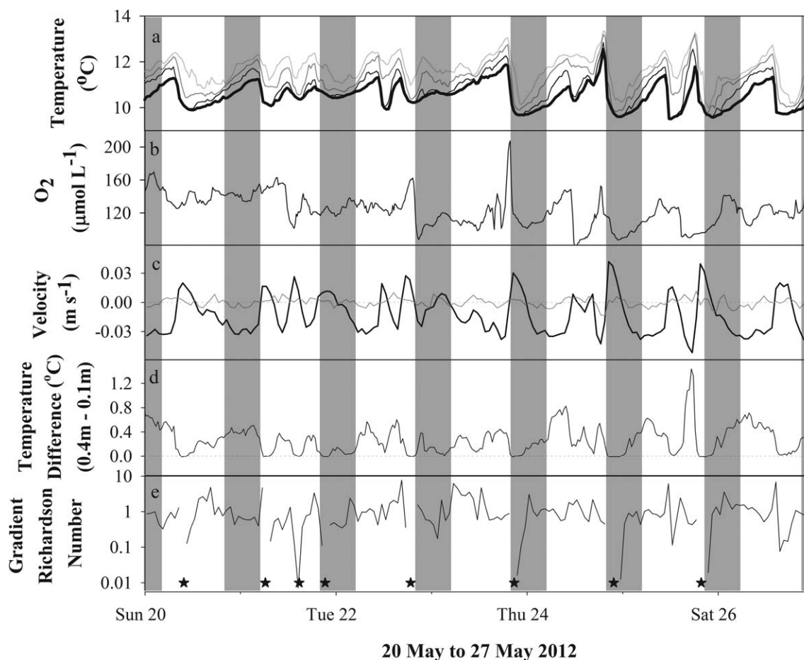
Fig. 3. Temperature measured at z=0.2, 0.4, 0.9 , and 1.3 m from darkest line to lightest line, respectively (a), dissolved oxygen measured at z=0.1 m (b), hourly mean along and across lake velocities (along lake velocity in black and across lake velocity in gray, (c), temperature difference between z=0.4 m and z=0.1 m (d), and gradient Richardson numbers (e) within the bottom boundary layer between 20 May 2012 and 27 May 2012. Gray bars represent the period from sunset to sunrise. Positive velocity values indicate upslope flow for along-lake velocities and flow toward the northeast for across-lake velocities. Unstable stratification events are marked by stars in panel (e), and associated gradient Richardson numbers are not plotted due to log scale.
