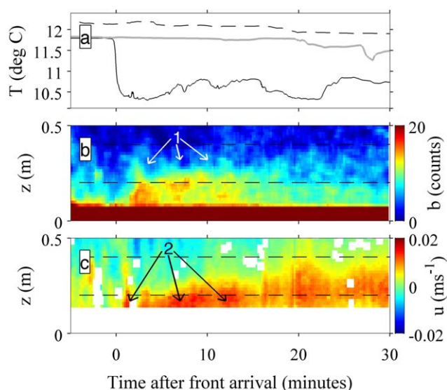
Fig. 5. Arrival of a thin bore. Panel a: Temperature measured 0.1, 0.4, and 0.9 m above the bed (respectively thin black, thick gray, and dashed lines). Panel b: acoustic backscatter b , with trends resulting from beam spreading and attenuation removed. Panel c: upslope water velocity. Horizontal dashed lines in panels b and c indicate elevations of temperature gauges. The arrival of the thin bore (marked by sudden near-bed temperature drop, panel a), was followed by elevated near-bed backscatter (labeled 1 in panel b), and slow upslope water velocity within 0.2 m of the lakebed (labeled 2 in panel c).
