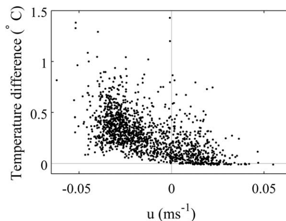
Fig. 4. Stratification (temperature 0.4 m above bed minus temperature 0.1 m above bed) vs. upslope water velocity. Each data point is a 1 h average, all 1430 h of good data shown.
