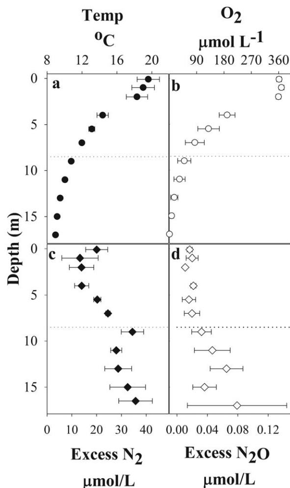
Fig. 2. Average profiles of temperature (a), dissolved O_2 (b), excess N_2 (c), and excess N_2O (d) at the deep water site between 30 May and 26 July. The dotted line indicates the depth of the internal shoreline tripod. Standard error bars shown ( n = 5 ).
