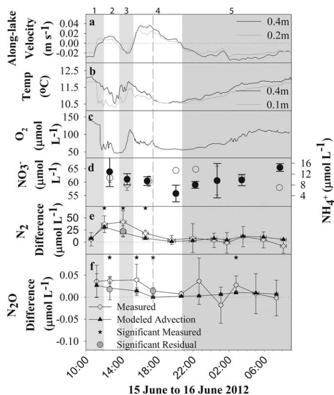
Fig. 6. Along-lake velocity (positive values indicate upslope flow, (a), temperature (b), dissolved oxygen concentrations at z = 0.1\text{ m} (c), mean NO_3^- (hollow circles) and NH_4^+ (black circles) concentrations (d), N_2 concentration differences (e), and N_2O concentrations differences (f) within the BBL over a 23 h wave period. In (e) and (f), hollow diamonds show total measured concentration differences whereas black triangles show the advection-based concentration differences based on temperature modeling. Black stars indicate measured concentration differences that were statistically different from zero (one sample t -test, p < 0.05 ). Gray circles show significant residual concentration differences (where measured and modeled vertical concentration difference were significantly different by t -test, p < 0.05 ). Gray dashed line demarcates the collapse in BBL thermal stratification. Five subintervals are also specified at the top of the figure: (1) arrival of thin bore, (2) sheared upslope flow, (3) small shear and no trend in stratification, (4) strongly sheared upslope flow, and (5) downslope flow. 95% confidence intervals shown.
